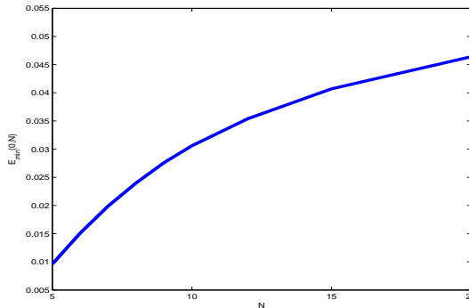
Figure 13: E_{\min}(0, N) for N \in [5, 20]
