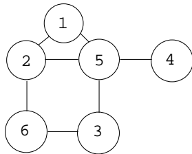
Figure 5: Aggregate sparsity pattern
