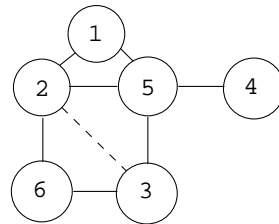
Figure 6: Extended sparsity pattern
